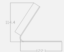
Desktop Bracket
